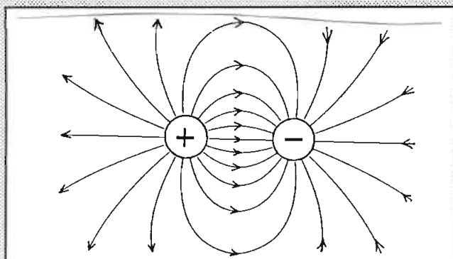
Ordinary electrical charges produce field lines that spread to infinity throughout the aether ('empty space').
